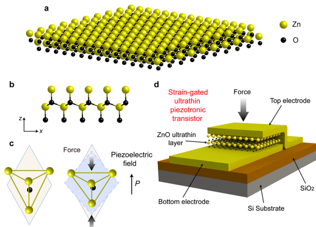
Figure 1. Strong out-of-plane piezoelectricity in ultrathin ZnO material with wurtzite structure for ultrathin piezotronic transistors. (a) Ultrathin ZnO materials with wurtzite structure. (b) View of the ZnO structure from the side. (c) ZnO nanomaterials with a hexagonal structure consisting of Zn–O–Zn stacking, with the O atom centered in the tetrahedron (left). A piezoelectric field points along the c -axis when the unit cell of ZnO nanomaterial is compressed by external force in the z -direction (right). (d) Schematic illustration of an ultrathin piezotronic transistor with two-terminal configuration. The stress-induced strong out-of-plane piezopotential in ZnO ultrathin film can effectively modulate the metal–semiconductor barriers to control the carrier transport.
