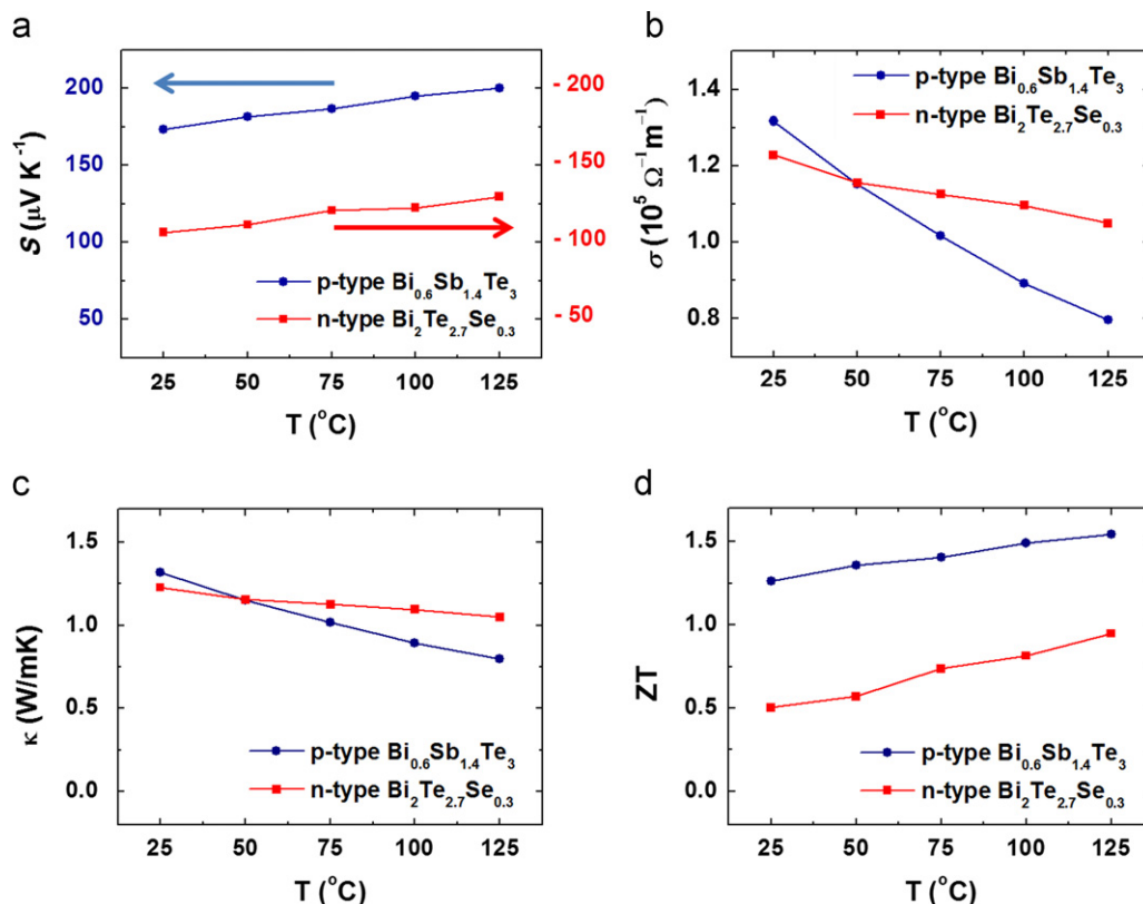
Fig. 2 Measurement of thermoelectric properties of p-type \text{Bi}_{0.6}\text{Sb}_{1.4}\text{Te}_3 and n-type \text{Bi}_2\text{Te}_{2.7}\text{Se}_{0.3} . (a) Seebeck coefficient, (b) electrical conductivity, (c) thermal conductivity, and (d) ZT values.
