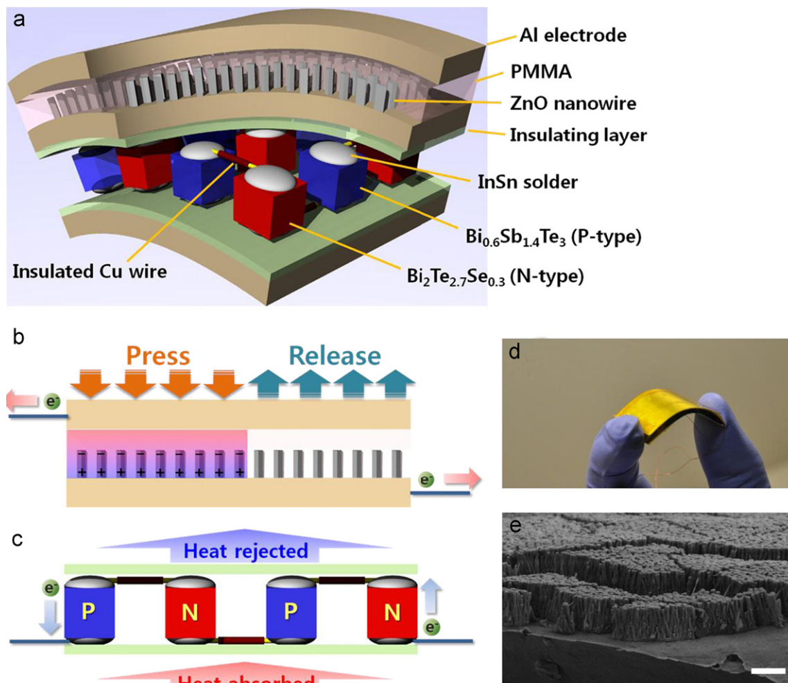
Fig. 1 Flexible HC, consisting of a NG above a TG. (a) Scheme of the vertically stacked hybrid device for simultaneously harvesting thermal and mechanical energies. (b) The working principle of NG. Positive/negative signs mean the polarity of the local piezoelectric potential created by an applied strain. (c) Electron flow diagram of the TG. (d) Photographic image of the flexible HC consisting of the TG and the NG. (e) SEM image of as-grown ZnO NWs on the thin Al substrate. Scale bar: 2 \mu\text{m} .
