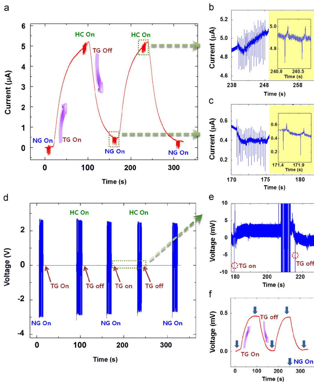
Fig. 4 The integrated performance of the HC under mechanically pressing and releasing with the increase of the temperature difference from 0^\circ\text{C} to 3^\circ\text{C} . (a) Output current when the TG and the NG are connected in parallel; and (b) and (c) enlarged view of the integrated output current of the HC. (d) Output voltage when the TG and the NG are connected in series; and (e) enlarged view of the integrated voltage of the HC. (f) Output voltage of the HC during mechanically pressing and releasing with disconnecting the electric wire to the NG and the measured value is similar to the result when we separately measured the output voltage of the TG.
