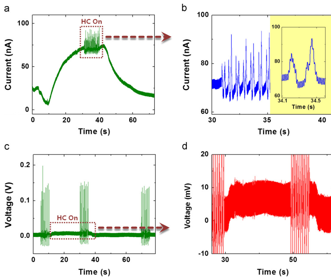
Fig. 5 The performance of the HC using skin temperature and body movement. (a) Output current and (b) enlarged view when the TG and the NG are connected in parallel, clearly showing that integrated output current is almost similar to the sum of the output of the two devices. (c) Output voltage and (d) enlarged view when the TG and the NG are connected in series.
